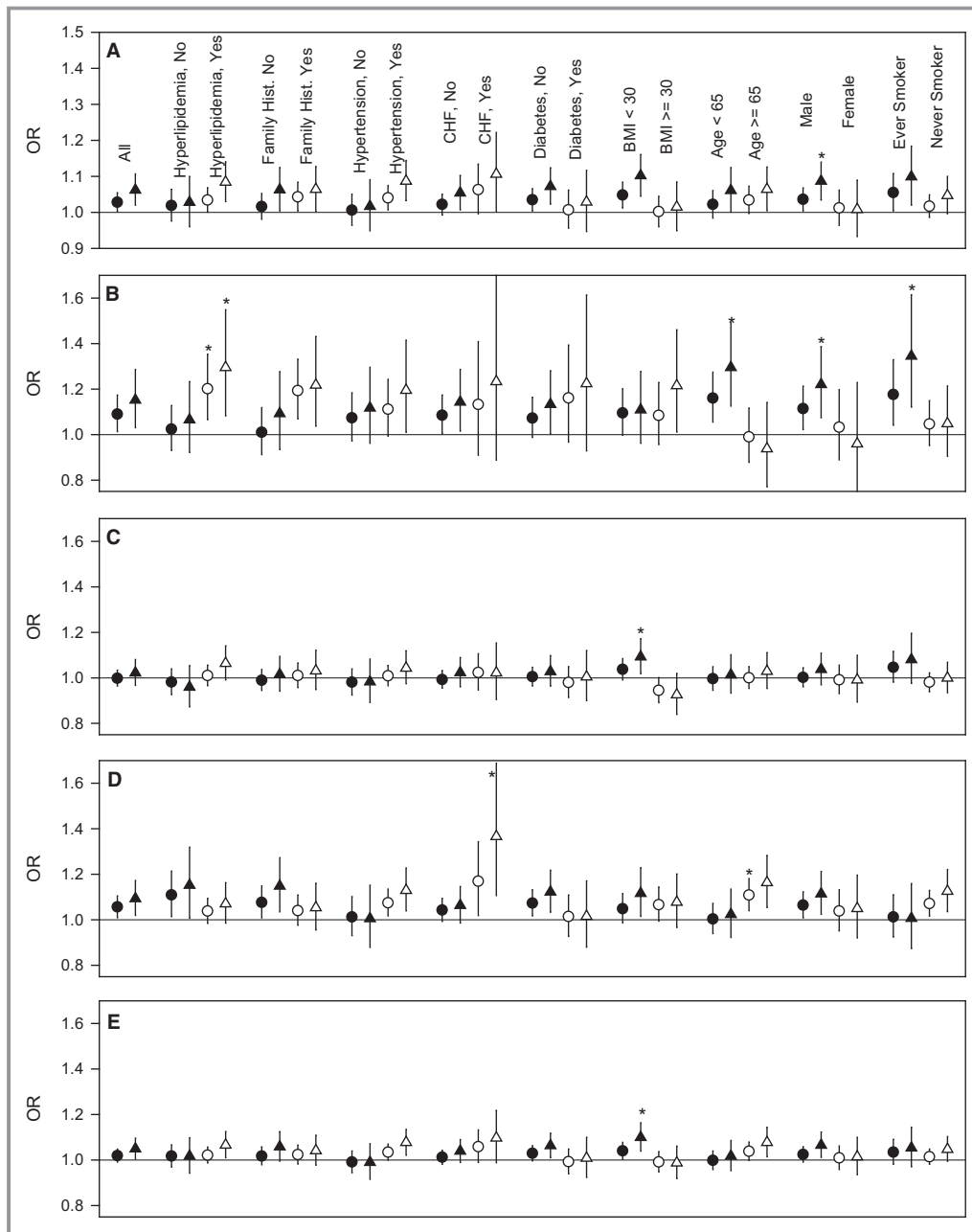
Figure 3. ORs (and 95% CIs) associated with a 10-µg/m 3 increase in PM 2.5 for all ACS (A), ST-segment elevation myocardial infarction (B), non-STEMI (C), unstable angina (D), and non-ST-segment elevation ACS (E) events for those with coronary artery disease across various strata. Circles represent results from the standard nonthreshold models, and triangles represent results from models with a PM 2.5 threshold of 25 µg/m 3 . *Strata with a statistically significant (P<0.05) larger effect vs the alternate strata. ACS indicates acute coronary syndrome; BMI, body mass index; CHF, congestive heart failure; Hist., history; OR, odds ratio; PM 2.5 , fine particulate matter ≤2.5 µm in aerodynamic diameter; STEMI, ST-segment elevation myocardial infarction.
